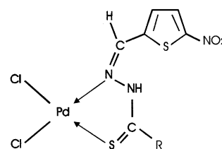
Figure 2. Structure of palladium(II) complexes: (1a) R = -NHC 7 H 7 ; (2a) R = -NHC 7 H 7 ; (3a) R = -NHC 7 H 7 ; (4a) R = -NC 5 H 12 ; (5a) R = -NC 8 H 10 ; (6a) R = -NHC 8 H 15 ; (7a) R = -NHC 10 H 15 ).
